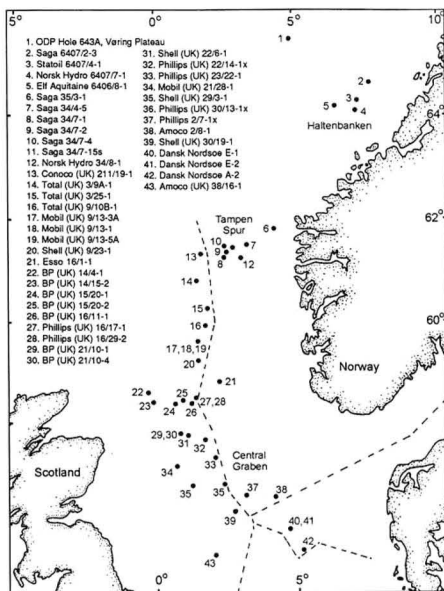
Fig. 1. Location of exploration wells in the North Sea and offshore Norway that recovered deep marine Palaeocene strata used to study the new agglutinated foraminiferal taxa.
