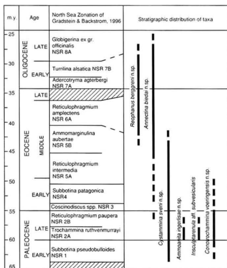
Fig. 13. Stratigraphical distribution of the new species in the Paleogene of the North Sea and offshore Norway. The zonation is after Gradstein & Bäckström (1996)
